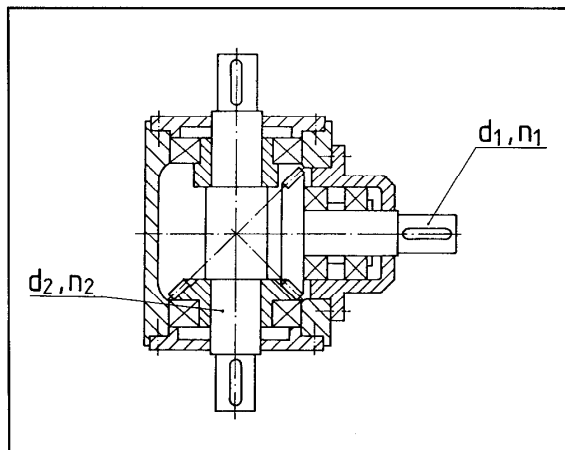
Vertical shaft arrangement
